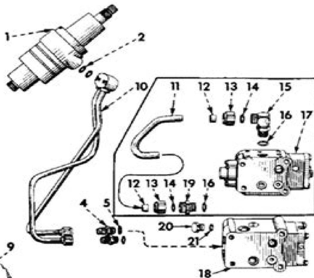
Tractors equipped with engine driven pump
