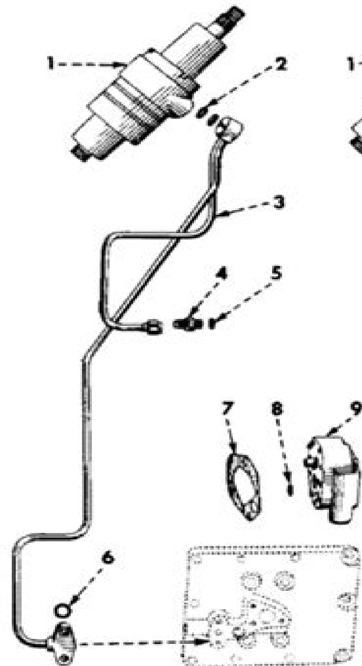
Tractors equipped with transmission driven pump
