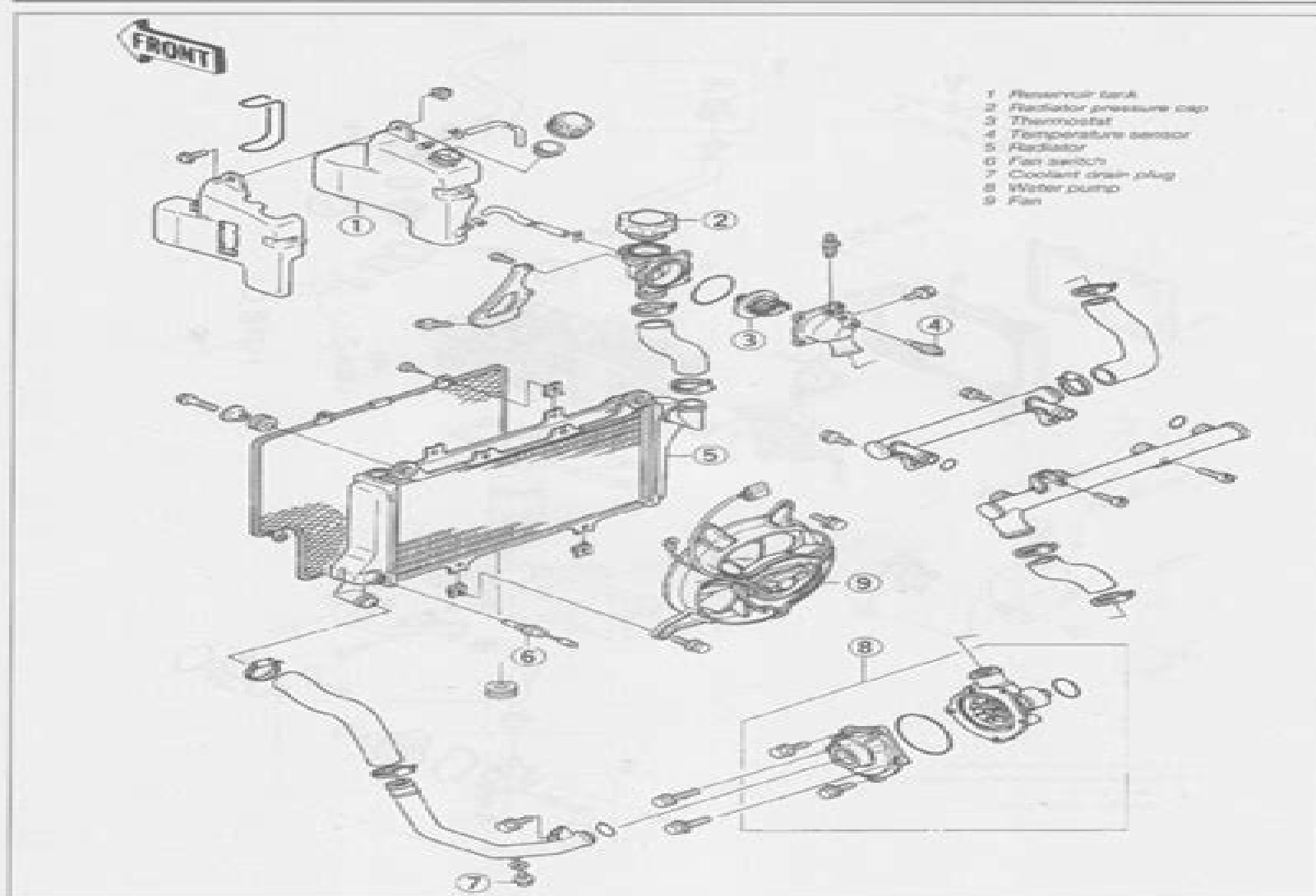
1.1c Exploded view of the cooling system (750 models)
