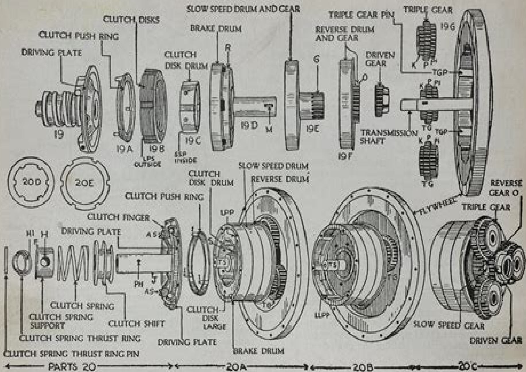
Fig. 29. Parts of the Ford transmission: The objects marked (19) to (19G) illustrate the parts of the transmission separated but in their respective order to be assembled.
