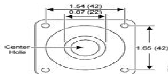
Figure 1: Mounting Holes on the Flange Dimensions in. (mm)
