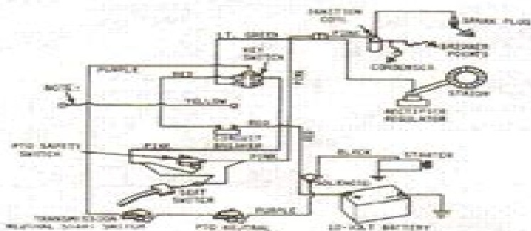
Fig. 10.103—Electrical wiring diagram for Model 2008
