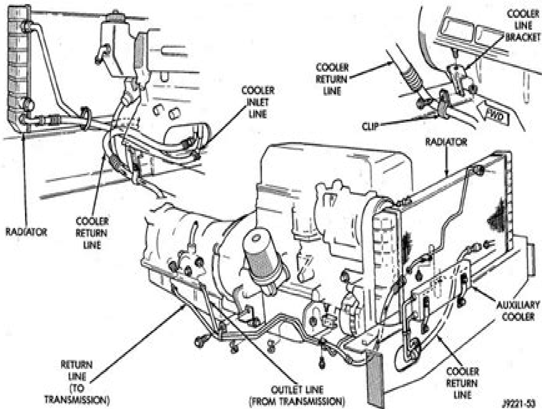
Fig. 48 Auxiliary Cooler Mounting (Left Hand Drive)
