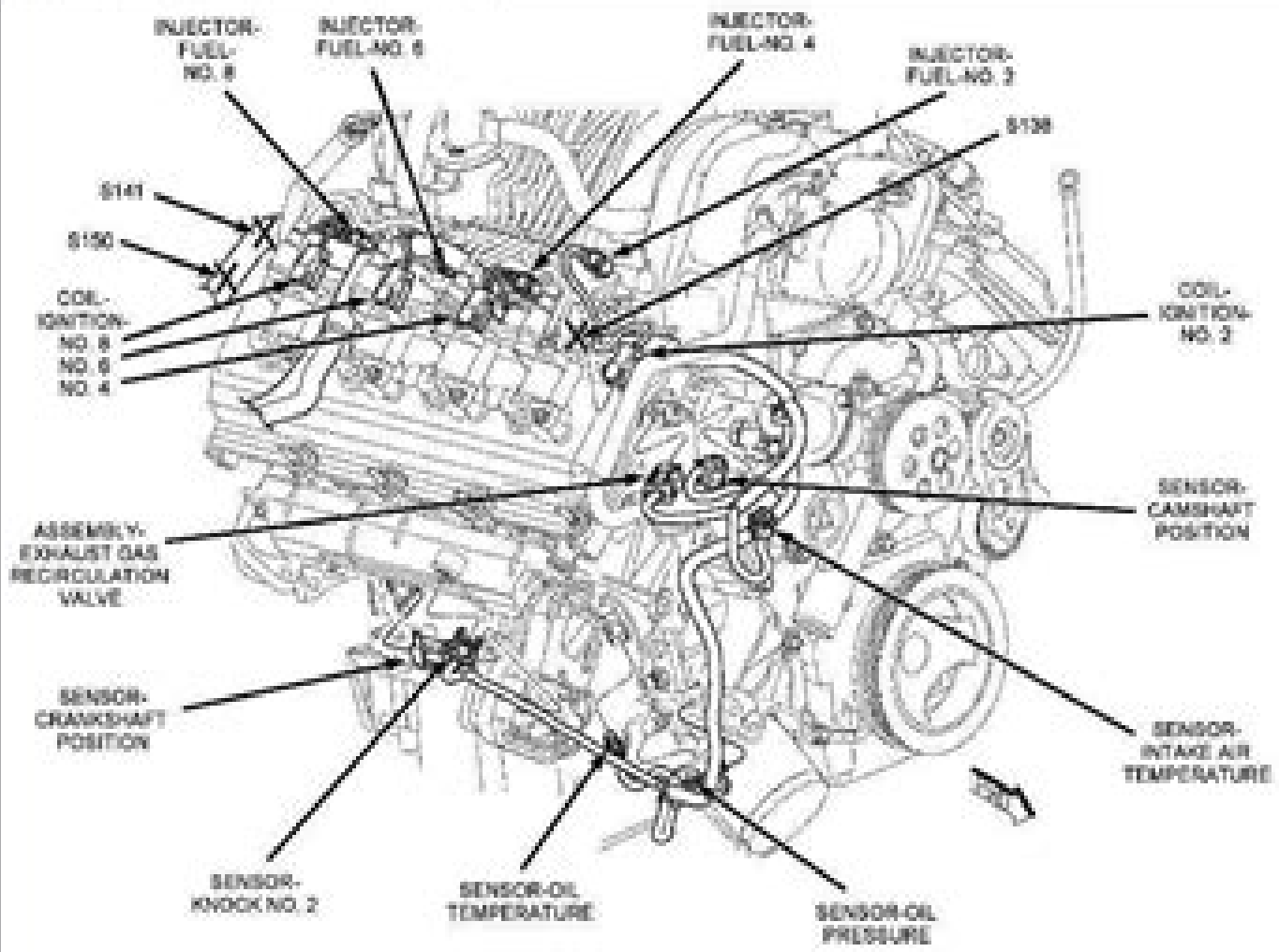
Fig. 24 LOWER RIGHT FRONT ENGINE (D 7L)
