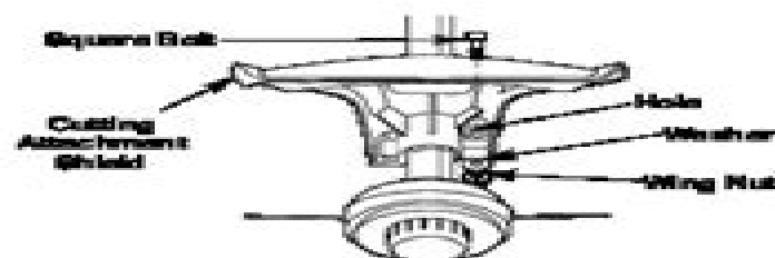
Cutting Attachment and Shield: Underside View
