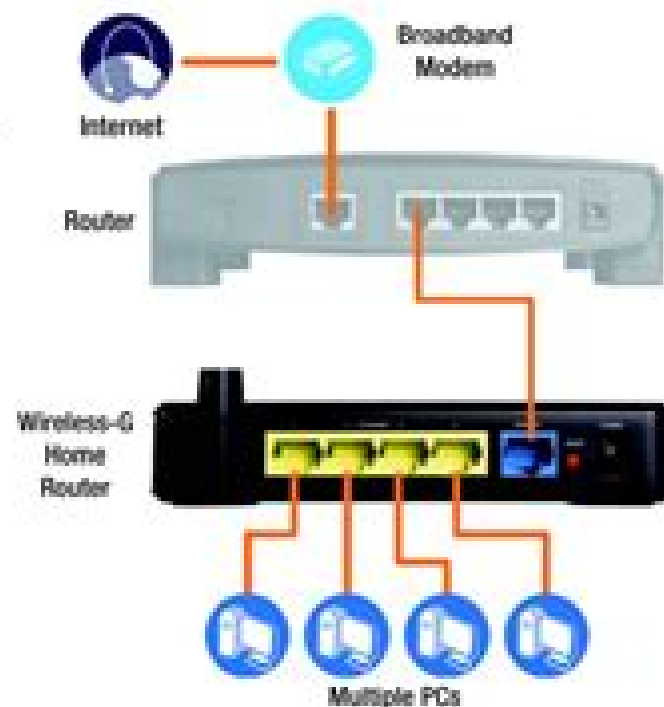
Figure 4-4: Diagram for Connection to Another Router
