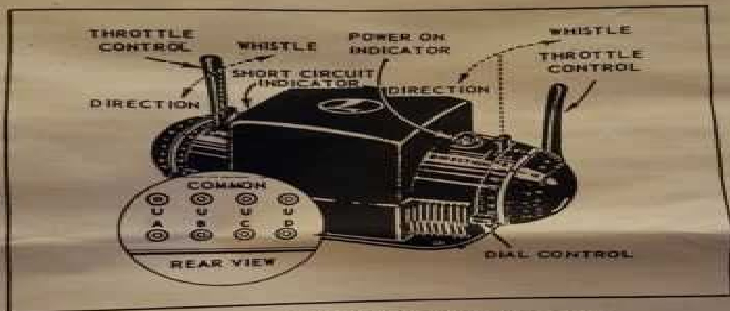
Figure 1 - Type ZW "Multi-Control" Transformer
