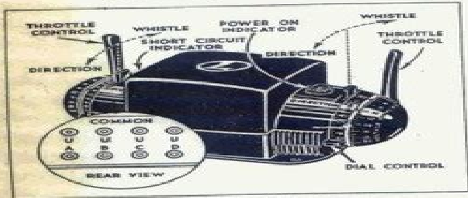
Figure 1—Type EW "Main-Control" Transformer.
