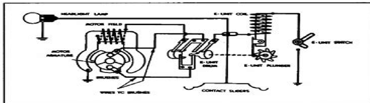
Figure 2 - Schematic Wiring Diagram of a Typical E-Unit Installation
