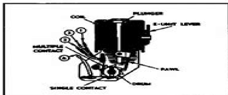
Figure 1 - Cross-section view of a E-Unit
