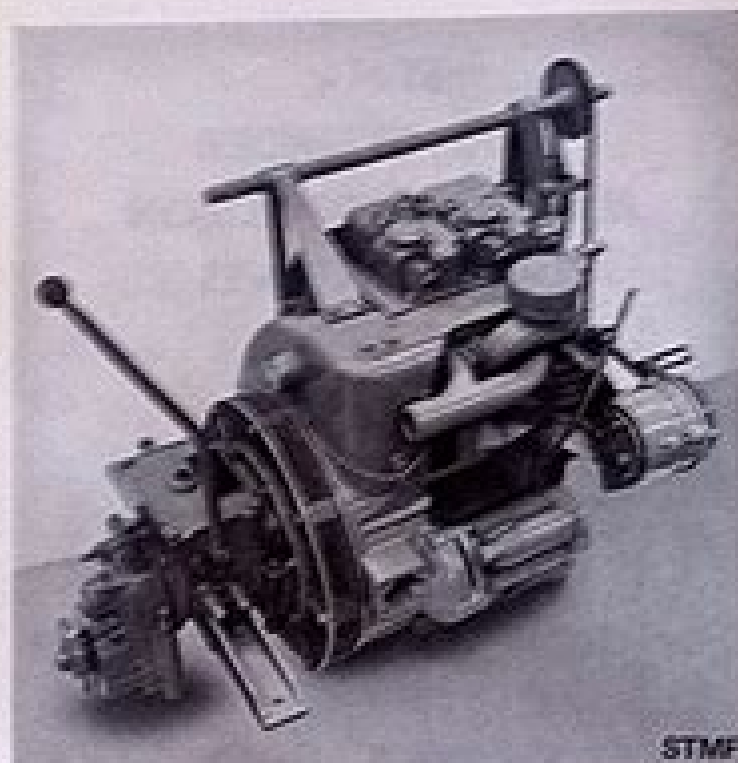
A Typical Lister STM Engine
