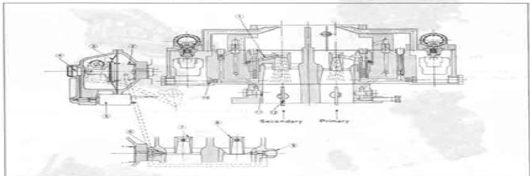
Fig. 4-3 Secondary circuit
