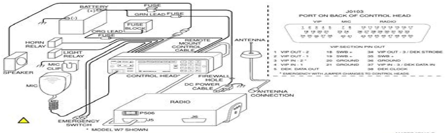
Figure 2-8. Radio Installation (Remote) Using W4, W5, W7, or W9 Control Heads
