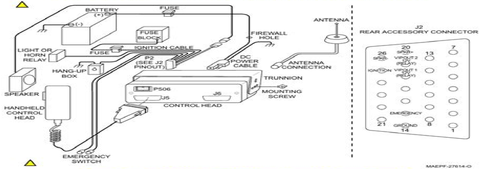
Figure 2-9. Radio Installation (Dash Mount) Using W3 Control Heads (For complete pin configuration, see Figure 3-9.)
