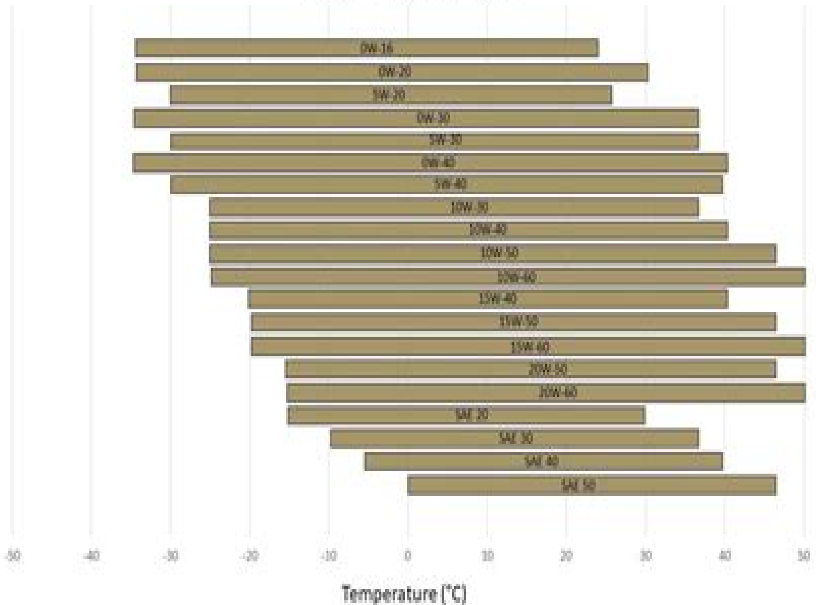
Viscosity Temperature Chart
