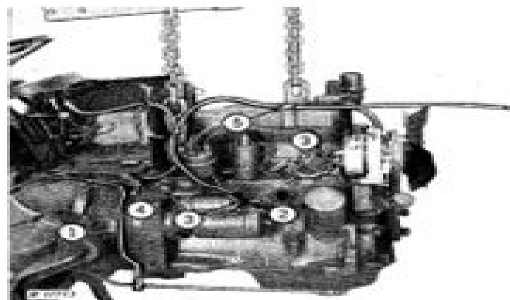
Fig. 10-Right-Hand Removal Procedure
