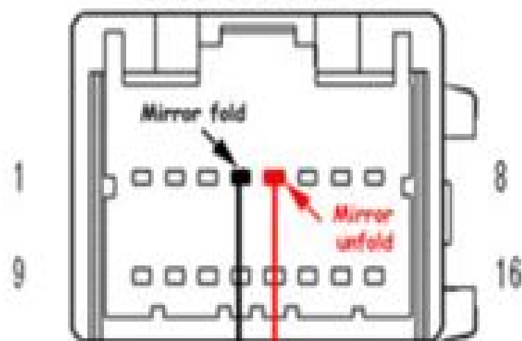
Driver's side mirror
