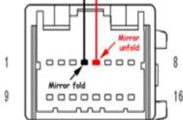
Passenger side mirror
