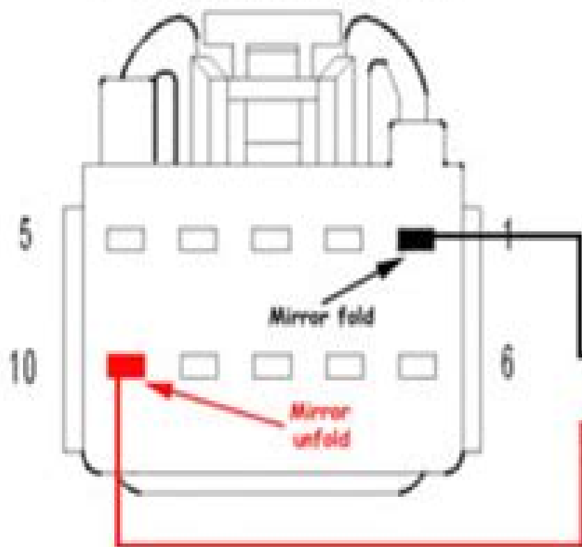
Power-folding mirror switch
