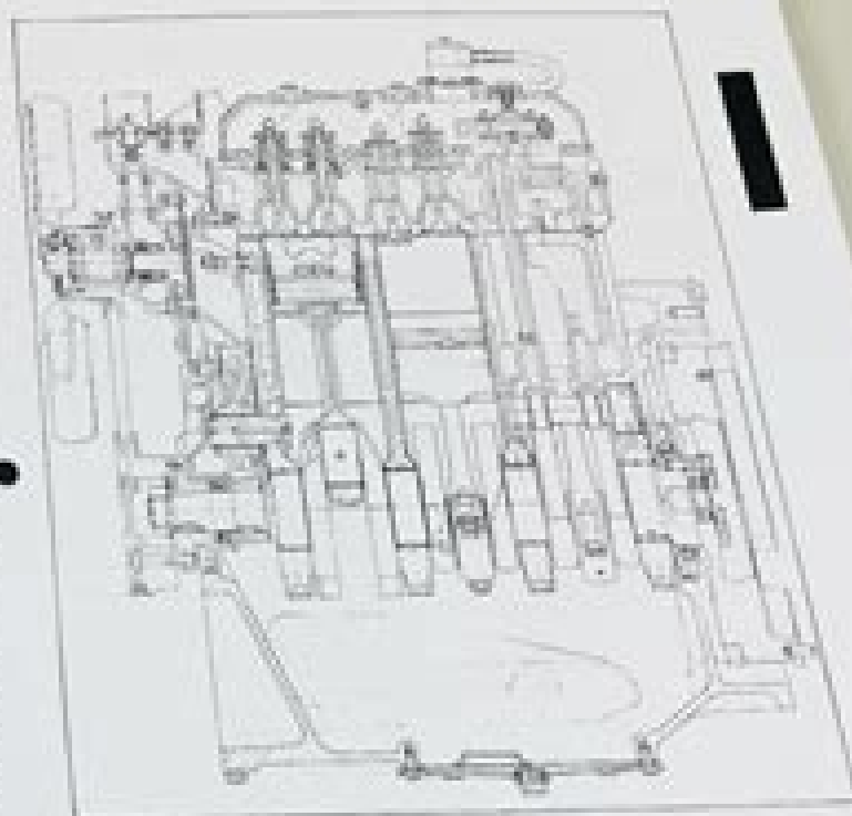
FIG. A.406 ENGINE - SECTIONAL VIEW
