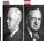
Cole 1936 Loree 1936
