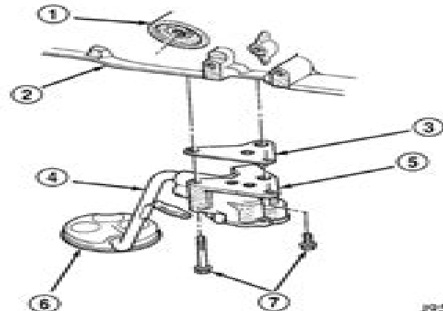
Fig. 82 Oil Pump Assembly
