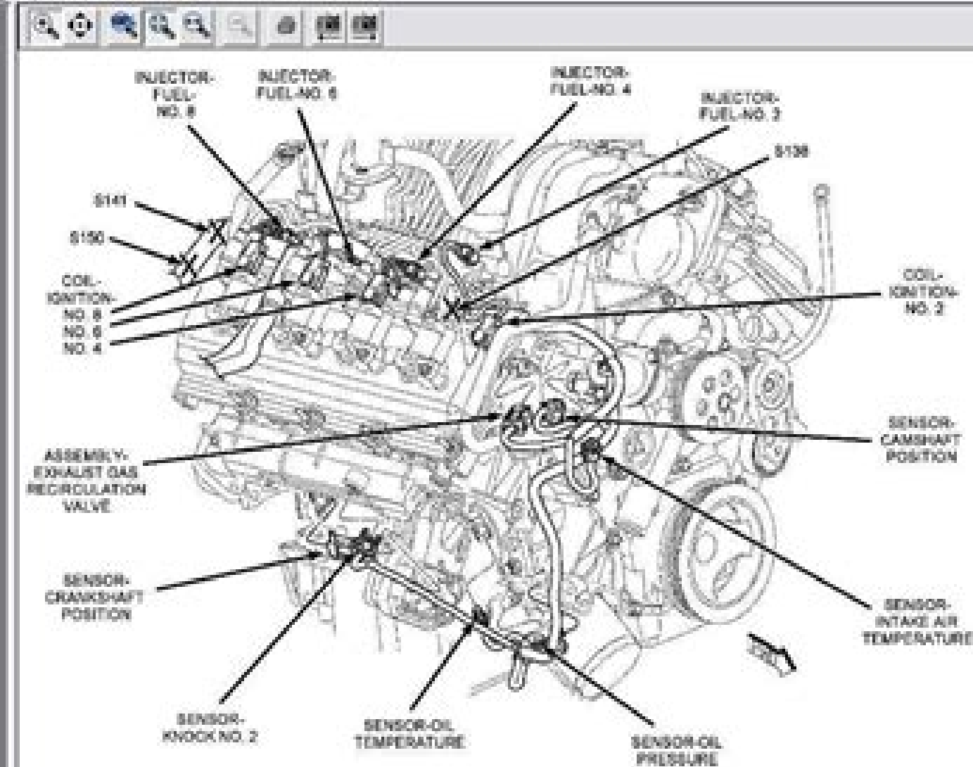
Fig. 24 LOWER RIGHT FRONT ENGINE (2.7L)
