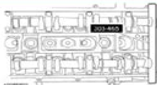
Fig. 38: Identifying Special Camshaft Tool (303-465) Courtesy of FORD MOTOR CO.
