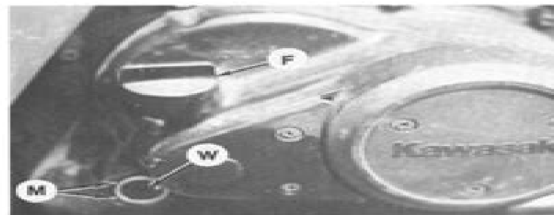
Fig. K4-1—Engine/transmission sump is filled through fill plug (F) opening. Oil level should be maintained between the two marks (M) next to level window (W).
