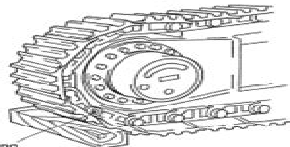
Fig. 34-3 Removing/fixing position of master pin
