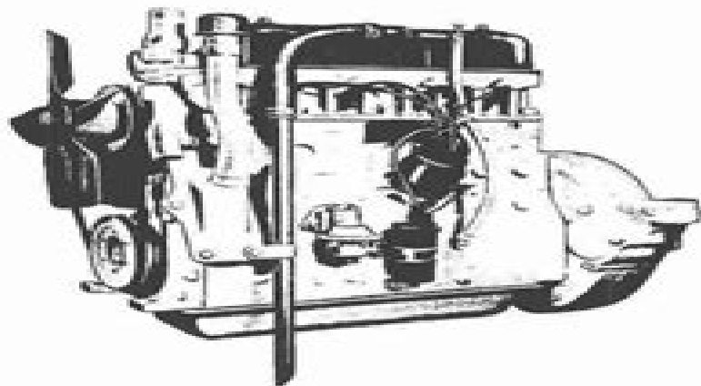
Figure 7 — G-4193 LH Side
