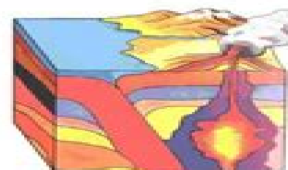
An example of contact metamorphism, where magma changes the type of rock over time
