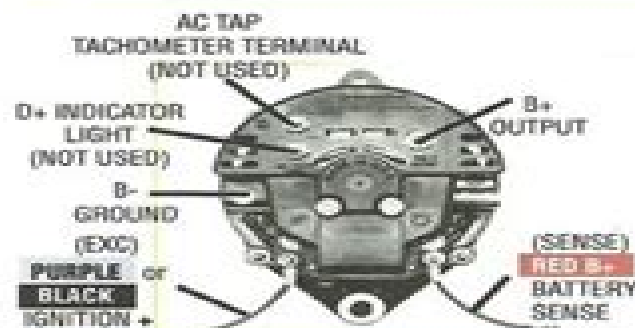
LATE MOTOROLA/PRESTOLITE STYLE FITS MERCURISER & OMC
