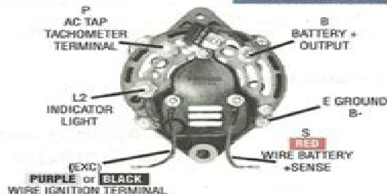
LATE MANDO STYLE FITS MERCURISER AND OTHERS
