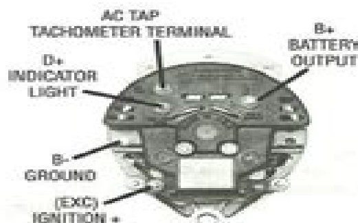
LATE MOTOROLA/PRESTOLITE STYLE FITS U.S. MARINE
