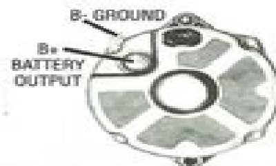
DELCO SELF EXCITING STYLE FITS MERCURISER AND OMC
