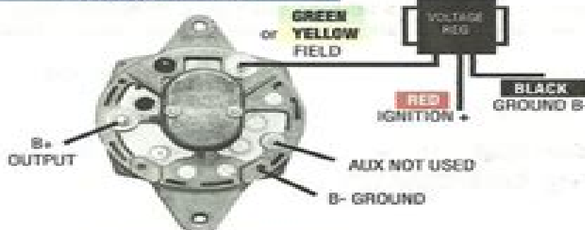
EARLY PRESTOLITE STYLE FITS OMC
