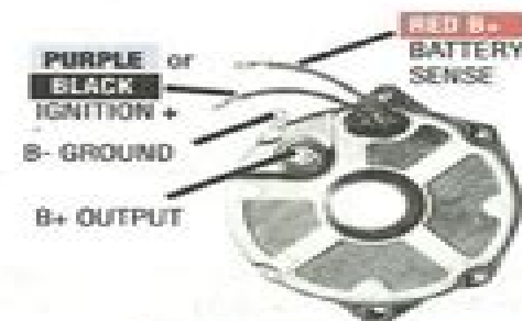
DELCO STYLE FITS MERCURISER & OMC
