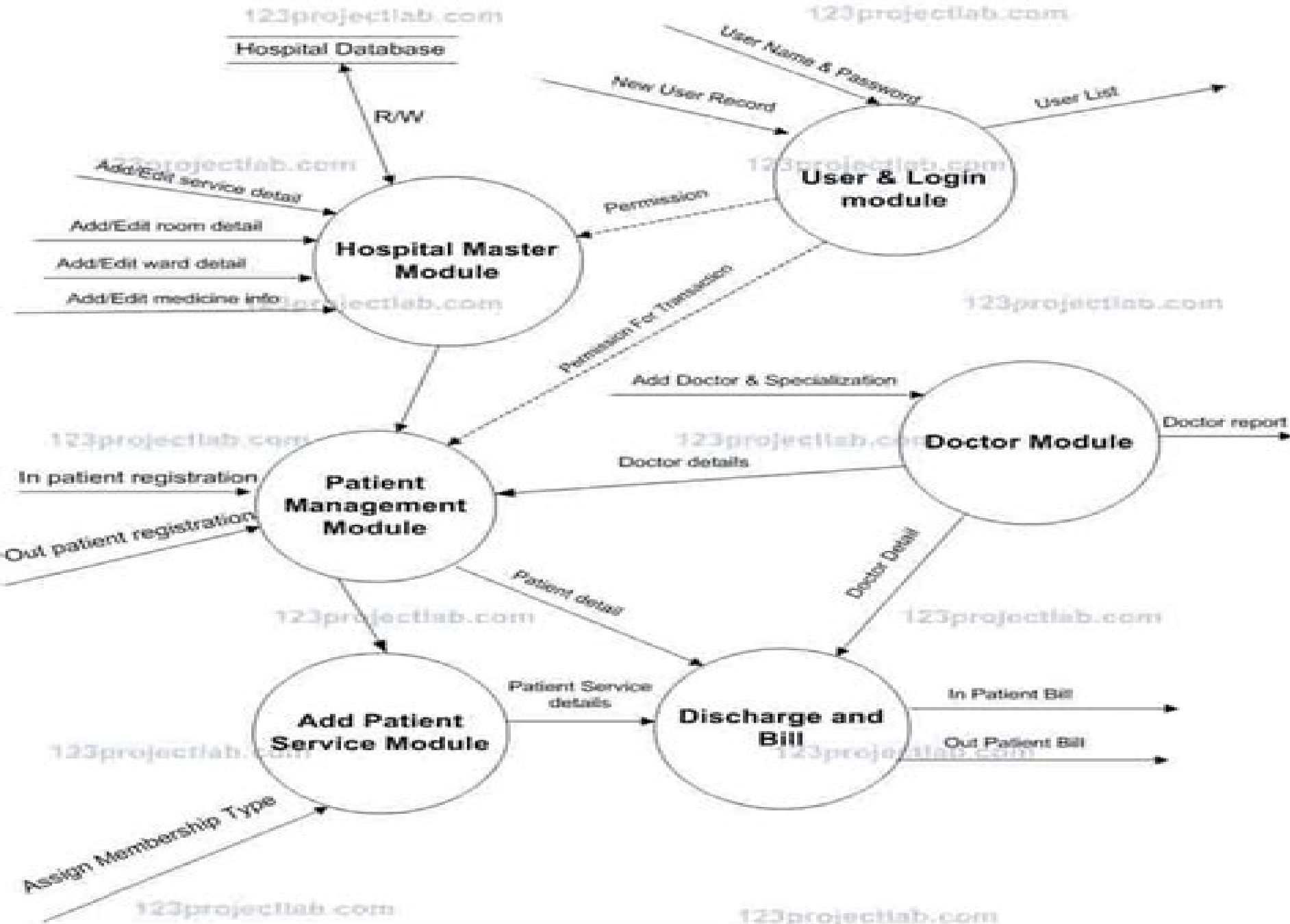
Level 1 DFD for Hospital Management System
