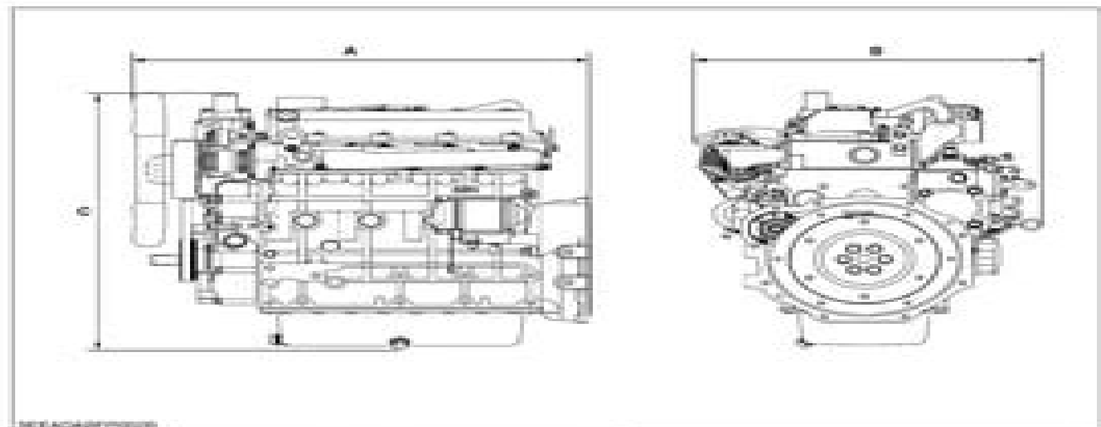
DETAILS (mm)
