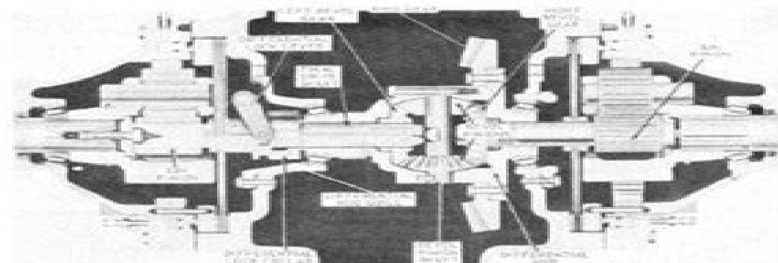
Fig. 165—Cross-sectional view showing the differential, differential lock and planetary reduction units devised on all tractors.
