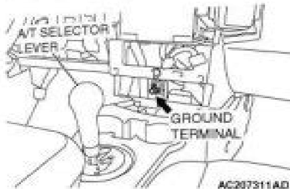
Fig. 47: A/T Selector Lever & Ground Terminal Courtesy of MITSUBISHI MOTOR SALES OF AMERICA.
