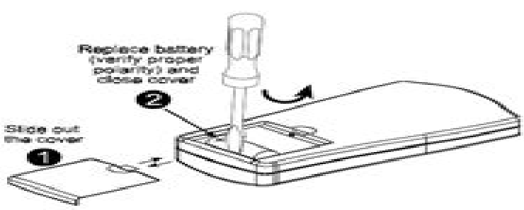
Figure 3 - Battery Replacement
