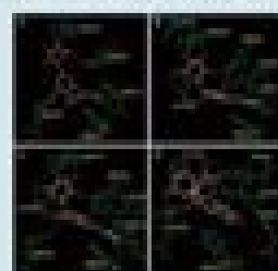
Fig. 2 Fluorescence spectra of Baocou (Baocou (I), Baocou (II), Baocou (III), and Baocou (IV)) under different conditions. The fluorescence spectra of Baocou (I) and Baocou (II) are represented using yellow dotted line. The spectra of Baocou (III) and Baocou (IV) are represented using red dotted line and blue dotted line, respectively.
