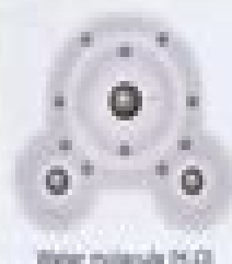
Water molecule ( H_2O )
