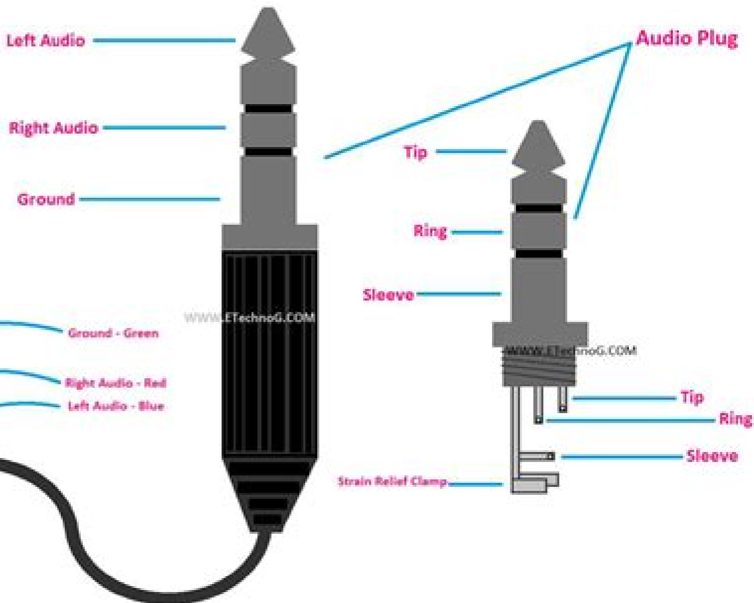
3 Pole or 3 Wire Headphone Jack Terminals(3.5mm Jack)
