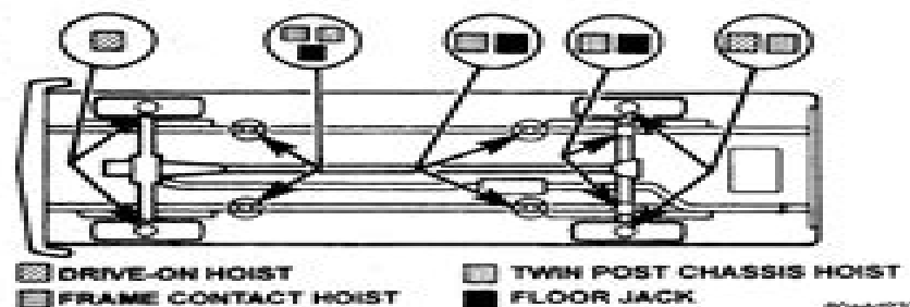
Fig. 5 Vehicle Lifting Locations
