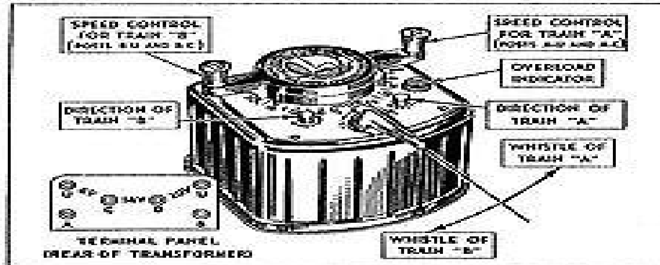
Figure 1—Type "KW" Multi-Control Transformer
