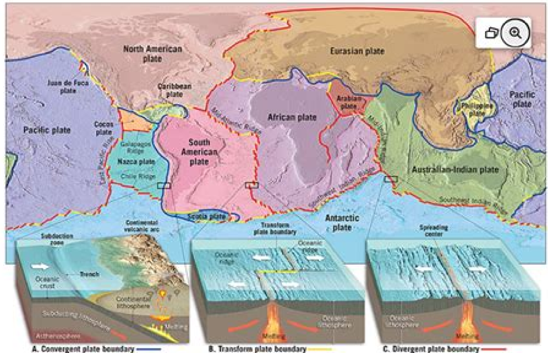
Figure 2.1 Earth's major lithospheric plates.
