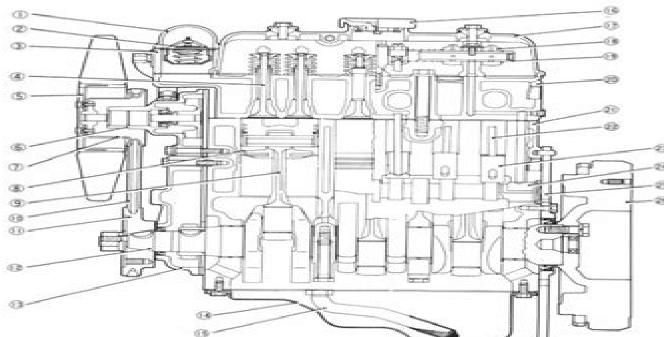
Longitudinal Sectional View of K3 Engine
