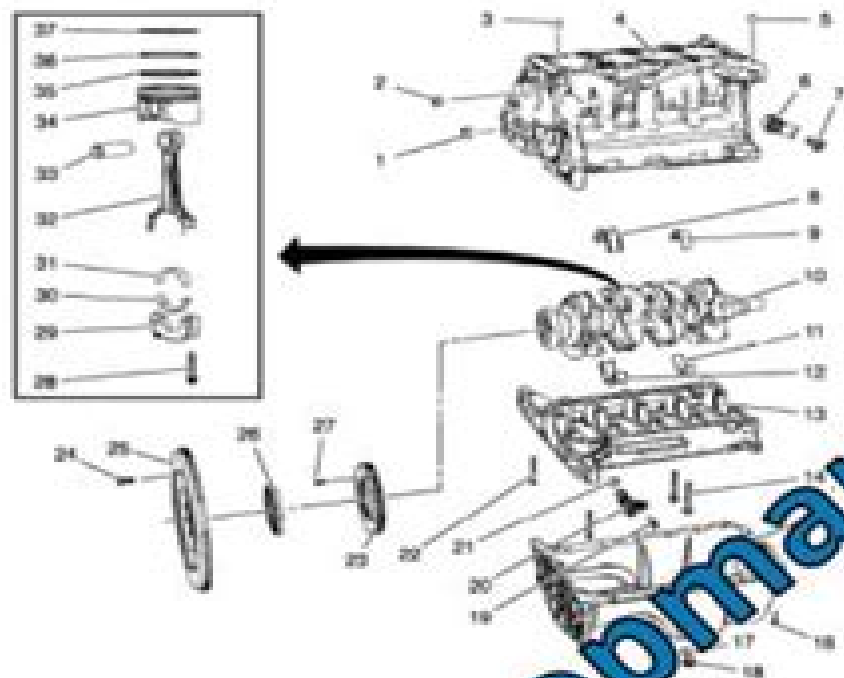
Fig. 7. Installing Engine Block Assembly Components
