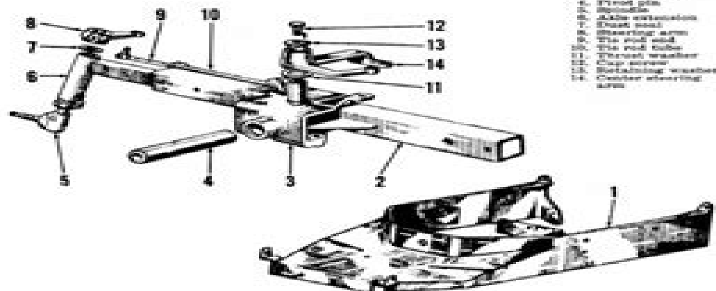
Fig. 1—Exploded view of engine frame, front axle, front support and associated parts used on Model MF25. Axle is similar on Model MF130, but cast front support bolts to cast iron oil pan and engine frame is not used. Refer to Fig. 2.
