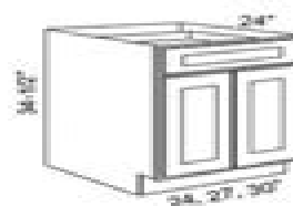
Double Door Bases B24, B27, B30
