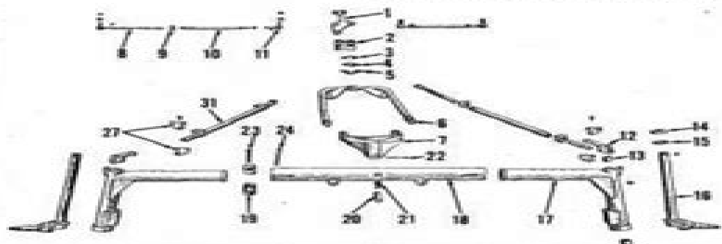
Fig. 4 - Exploded view of adjustable wide front axle used on Models 966 and 1066 Hi-Clear tractors.
