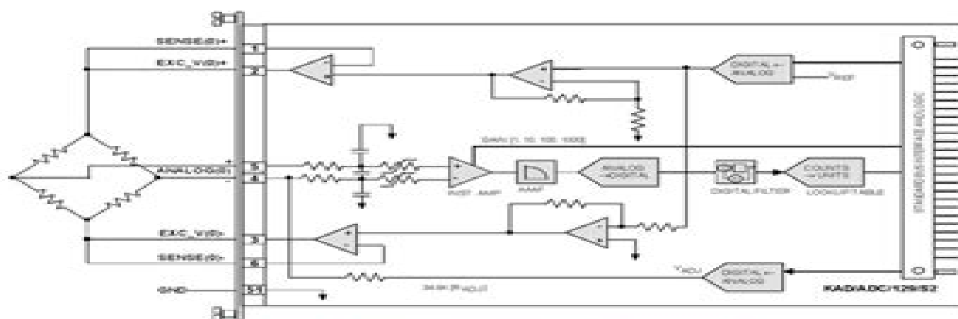
Figure 1: First of four channels on the KAD/ADC/120/52
