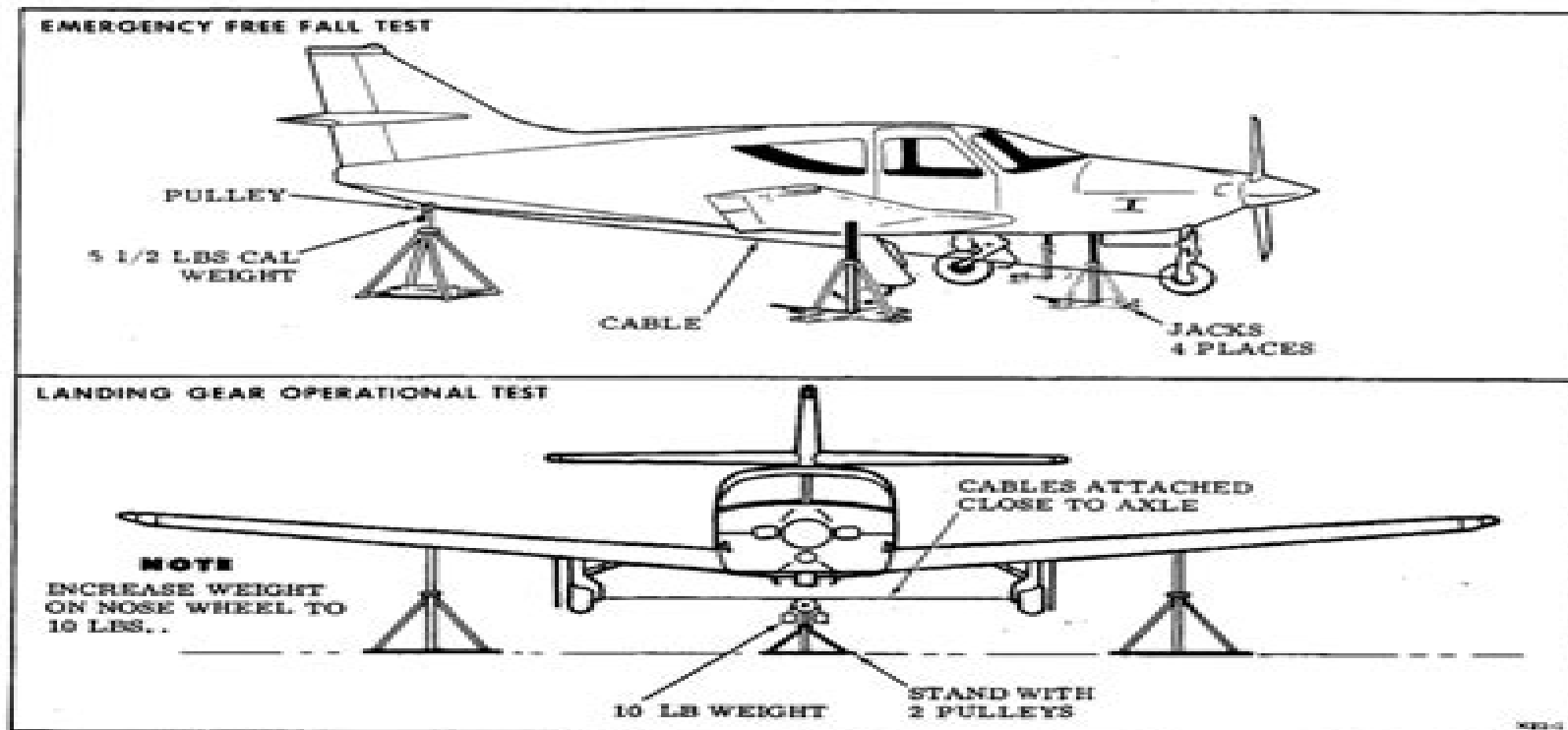
Figure 3-6. Hydraulic System Check
