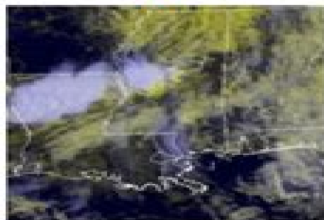
Multi-spectral Image
