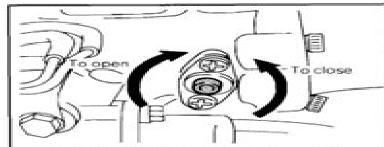
Fig. 10 — Variable intake control shaft
