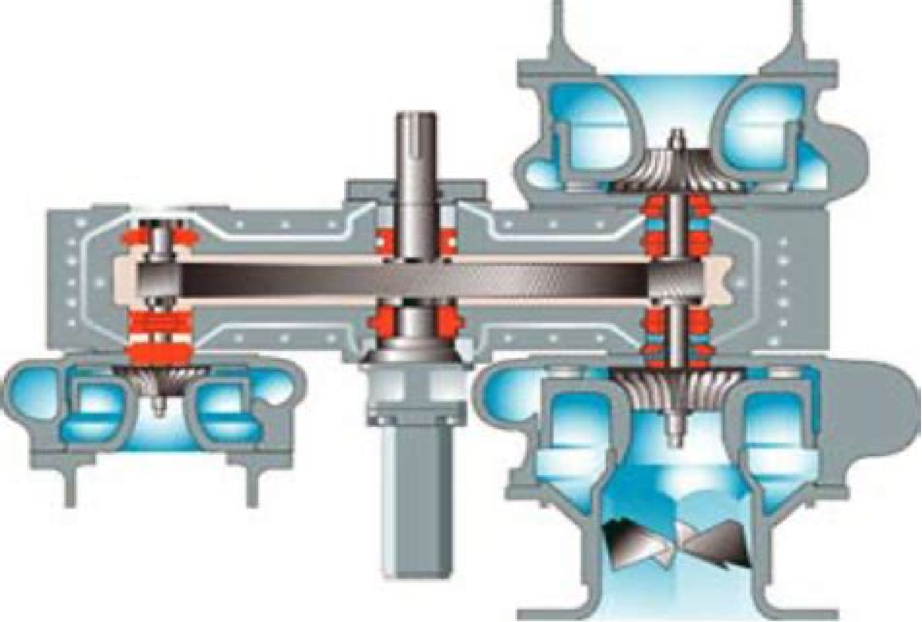
Three stage centrifugal compressor
