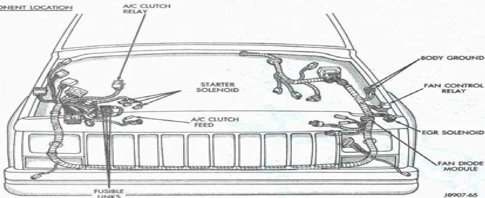
Fig. 42 Auxiliary Fan Controls—with A/C
